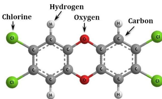
Most Toxic Dioxin: TCDD (2,3,7,8-tetrachlorodibenzo-p-dioxin)
